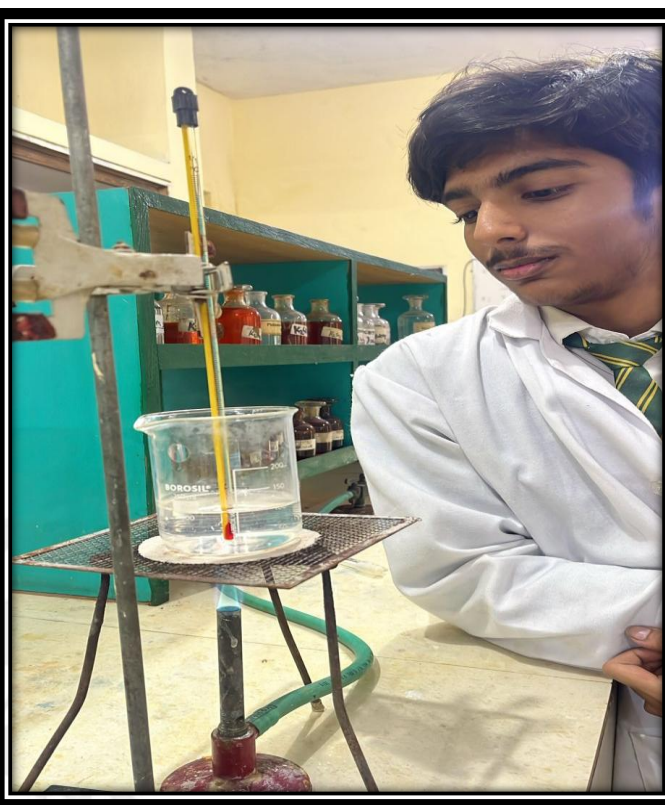
Elevation of Boiling Point
