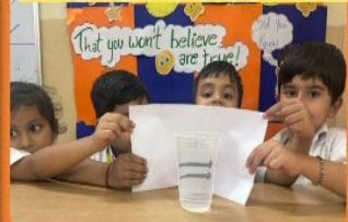
Reverse Refraction of light experiment
